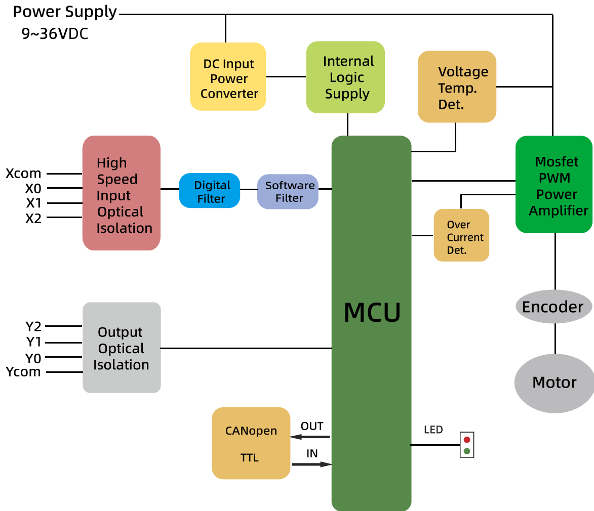
IM35EC-P Block Diagram
