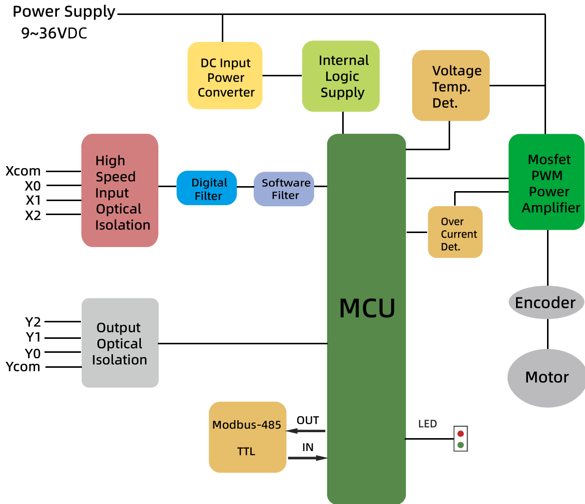
IM35ET-P Block Diagram
